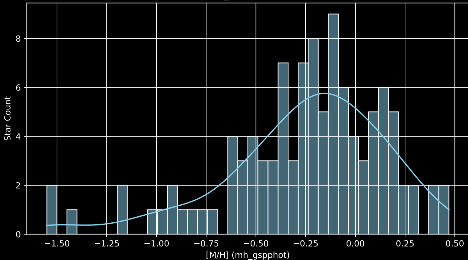
APOGEE DR17 Field: [357+05 [M/H] (mh_gspphot) (n= 106)
