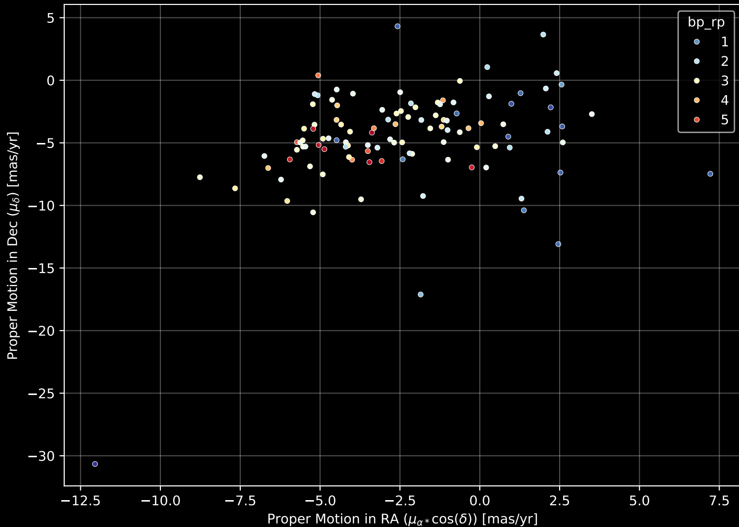
APOGEE DR17 Field: [357+05] Proper Motion Diagram (n= 110)
