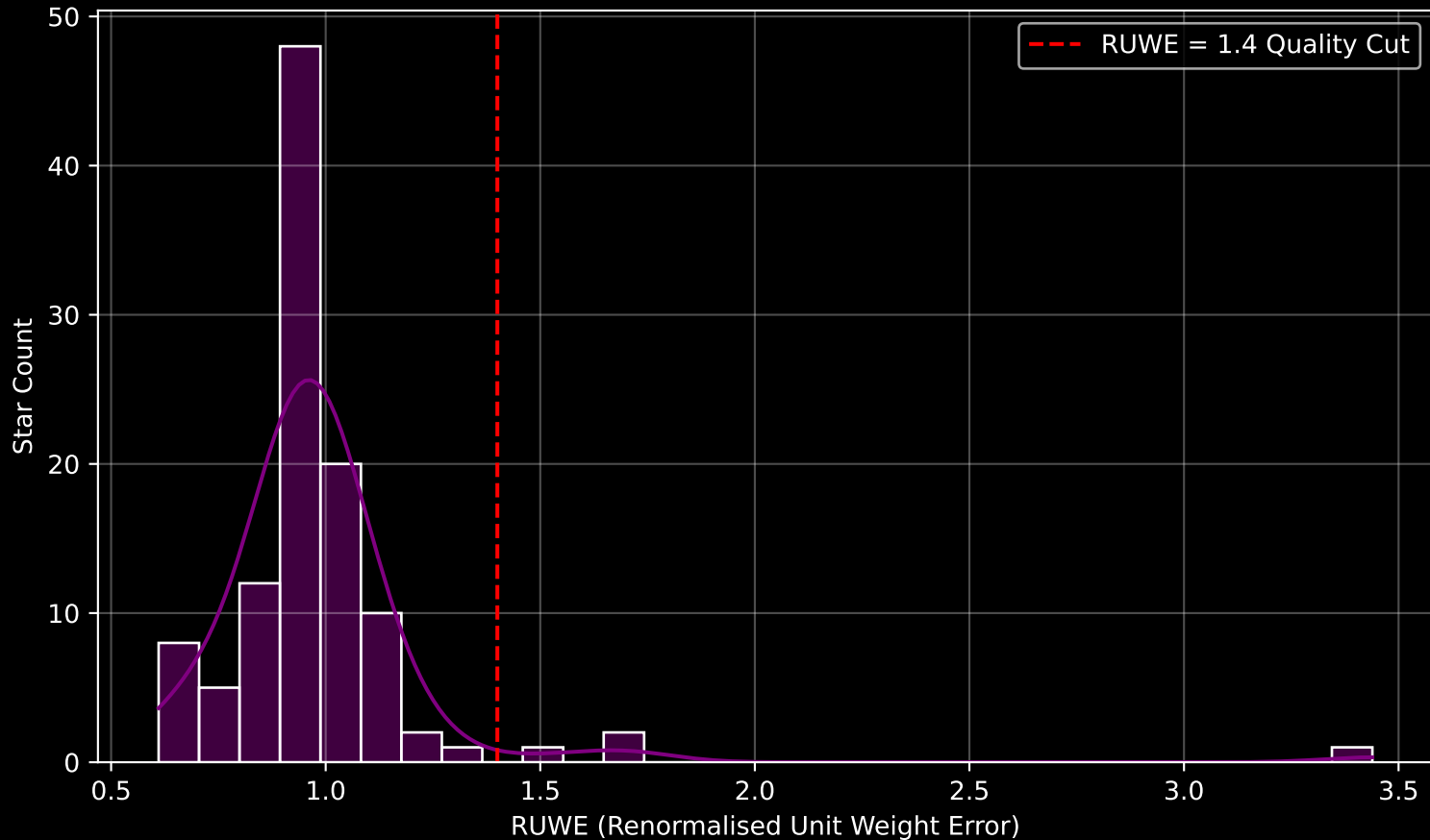
GAPOGEE DR17 Field [357+05] RUWE Distribution (n= 110)
