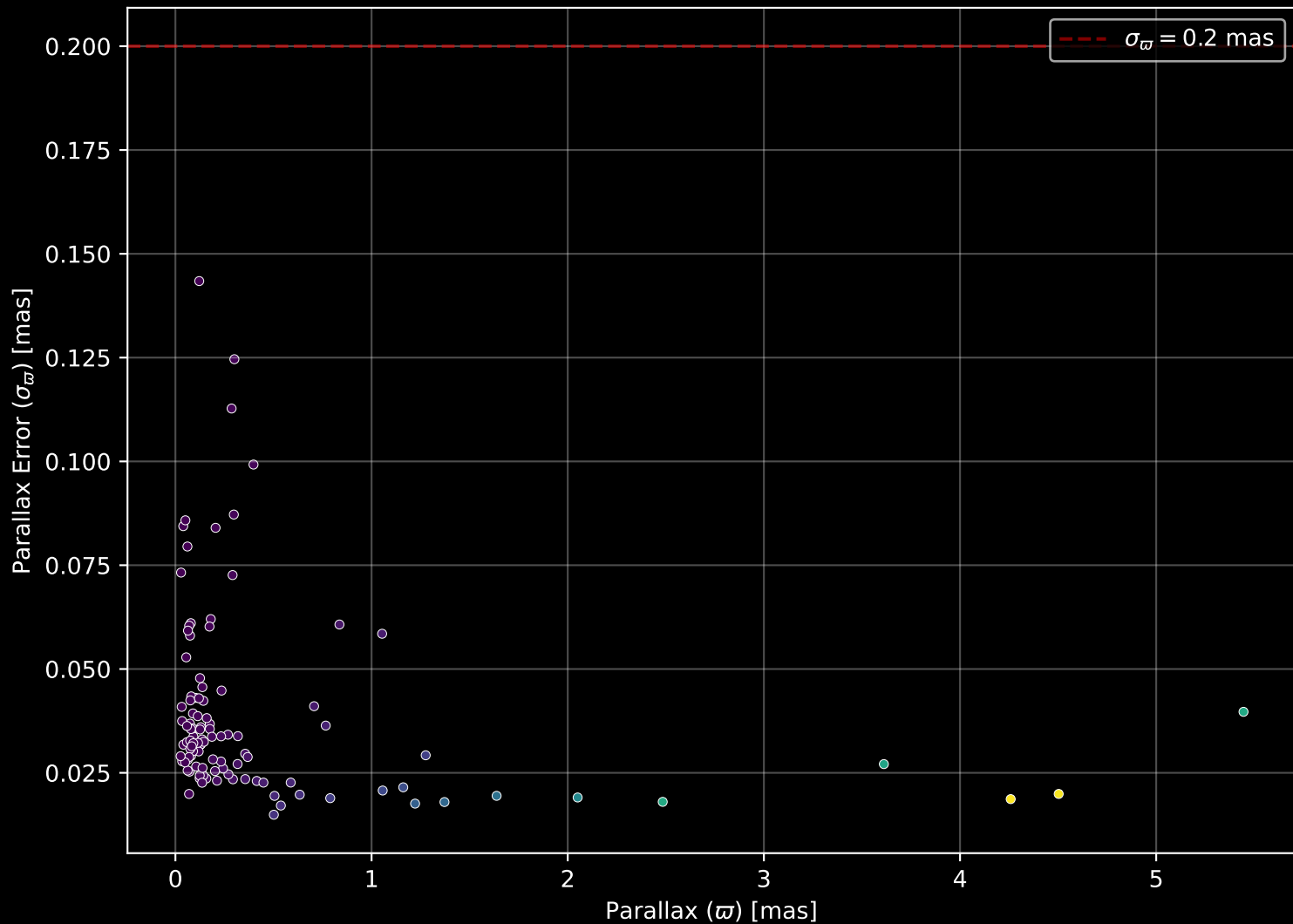
APOGEE DR17 Field: [357+05] Parallax Quality (n= 110)
