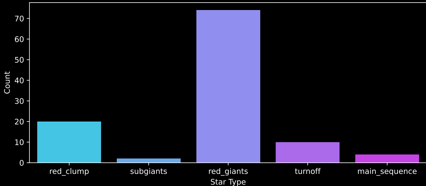
APOGEE DR17 Field: [357+05] Count plot of Star Type
